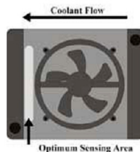
Figure 1c Cross Flow Radiator
